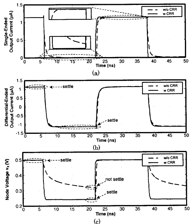
Fig. 6 (a) Single-ended output current, (b) differential-ended output current and (c) node voltage v_X of unit current cell.
