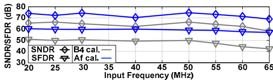
Fig.8. Measured SFDR &amp; SNDR vs. input frequencies.
