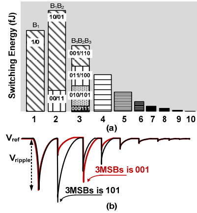
Fig. 2. (a) Switching energy v.s. digital outputs of an 11b SAR ADC. (b) Reference ripple during switching transients.
